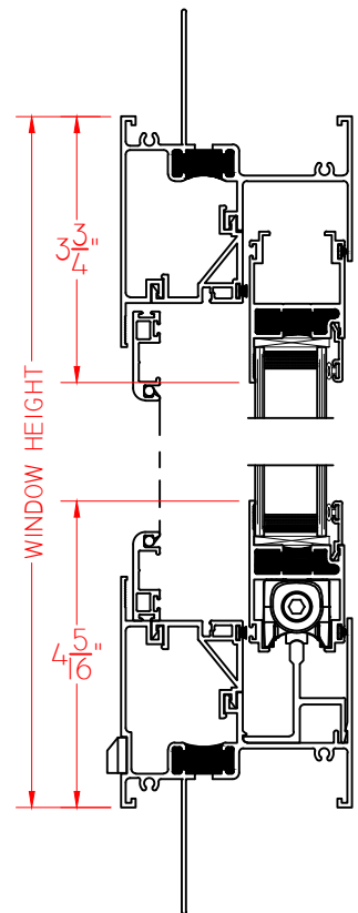
Ⓑ VERTICAL CROSS SECTION
