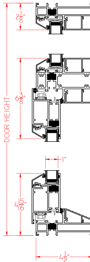
Ⓐ VERTICAL CROSS SECTION
