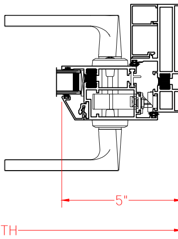
① HORIZONTAL CROSS SECTION
