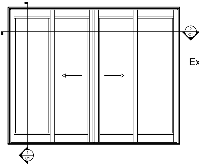
Window Elevation 3/8" = 1' 0"
