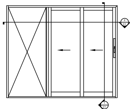
Door Elevation 1/4" = 1' 0"
