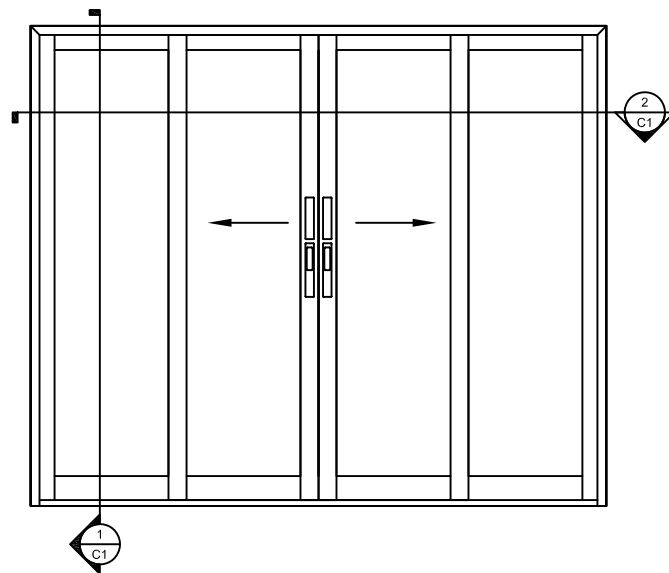
Window Elevation 3/8" = 1' 0"
