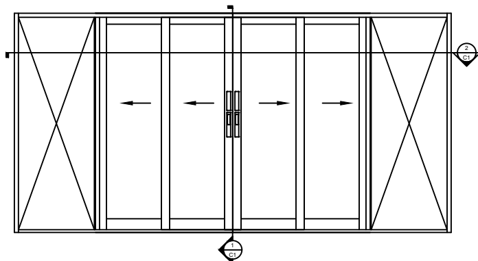
Door Elevation 1/4" = 1' 0"
