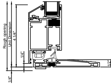
Low Profile Sill
