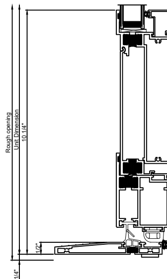
Low Profile Sill 10"
