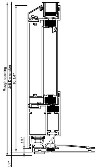
Low Profile Sill 10"
