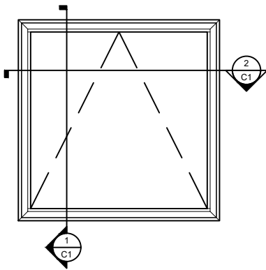
Window Elevation 3/8" = 1' 0"
