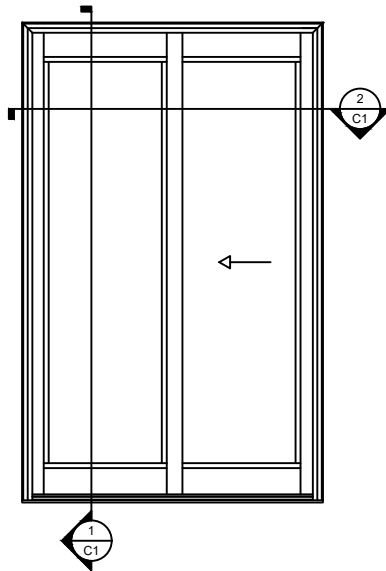
Window Elevation 3/8" = 1' 0"
