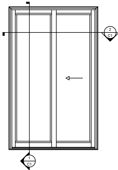
Window Elevation 3/8" = 1' 0"
